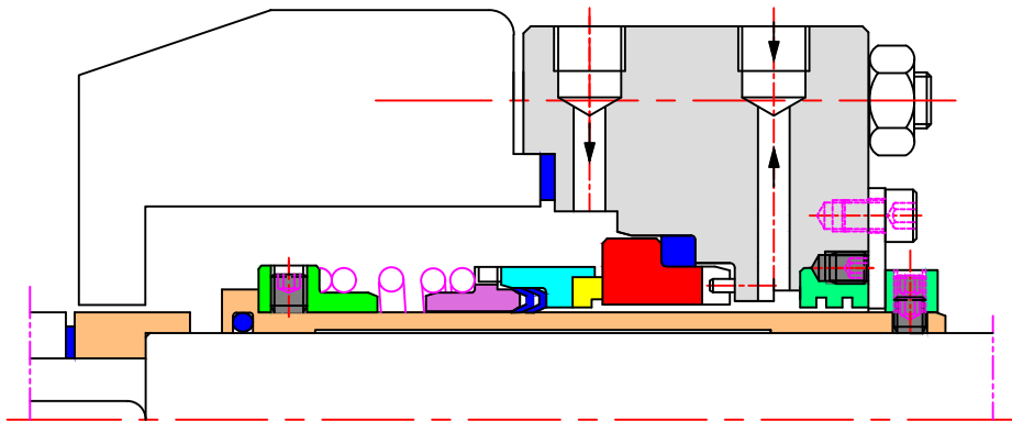
80 SERIES SINGLE SPRING MECHANICAL SEAL TYPE 8221 CARTRIDGE ARRANGEMENT WITH DIFFERENT API PLAN 11& 62
